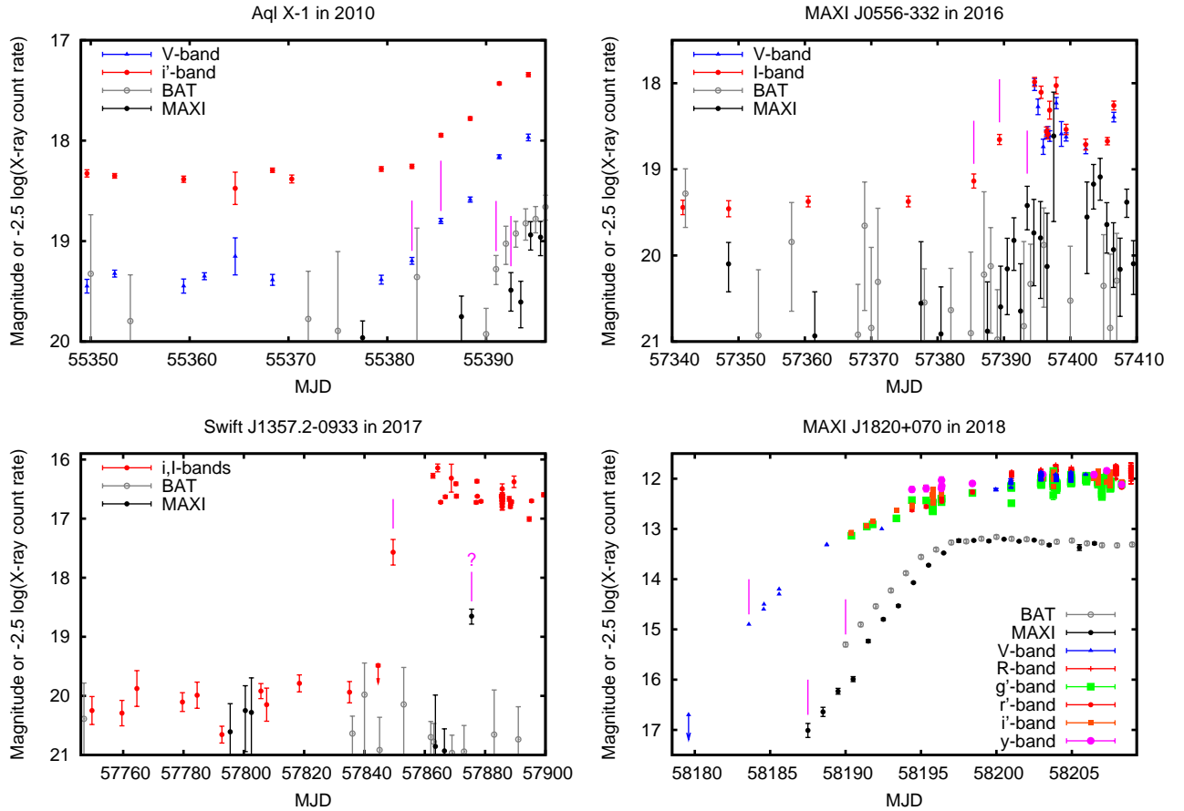
FIGURE 1 Examples of LMXB outbursts detected by optical telescopes before the first X-ray detections. Soft X-ray (2–20 keV) data from MAXI are shown in black and hard X-ray data (15–50 keV) from BAT on Swift are in grey. The purple vertical lines mark the dates of first significant detections at optical, then X-ray wavelengths. All were detected first with the Faulkes Telescopes except MAXI J1820+070, which was discovered as the optical transient ASASSN-18ey by the ASAS-SN survey.
